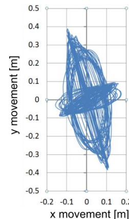
Figure 11. x-y position of platform shown as orbit paths (run 004_400_25).
