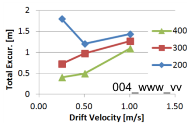
Figure 17. Plot of maximum platform excursion vs drift velocity for the 004_www_tt cases.
