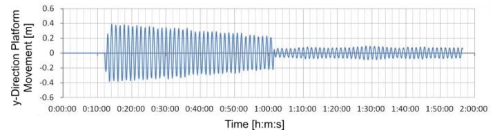
Figure 10. Time-history of platform movement in y direction (run 004_400_25).
